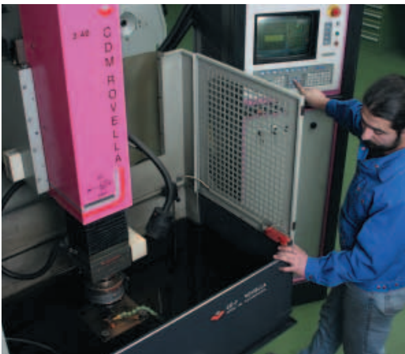
Drop-erosion-machine Rovella CDM and Eldis Astro 3.40 Zenit as well as a Wire-erosion-machine Charmilles Robofil 290 with a drilling machine Charmilles HD 8
